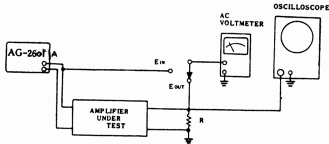
Fig. 2-1 Interconnections of the equipment.
